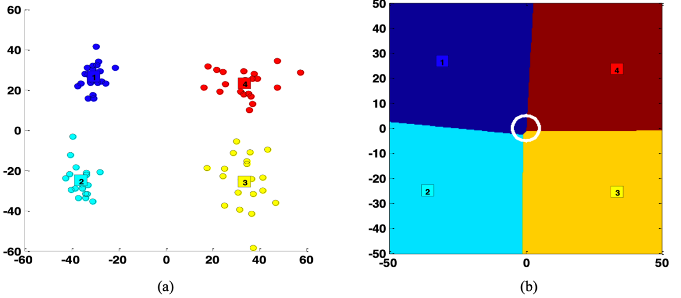
Figure 8. Results of the calibration of sensory interface using the total firing algorithms. The goal of the calibration procedure is to define the sensory regions by partitioning the position space of the controlled device. Here, we used a 4- box S_1 - M_1 network model and each time we stimulated one box, 20 times with different noise realization and hence we have 4 sets (cluster of points) which contains 20 points. (a): projecting the distance matrix, D , into in 2-dimensional space using MDS and (b) show the sensory regions obtained using a nearest neighbor algorithm. The squares show the centers of clusters.
